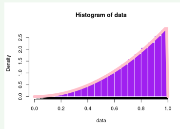
Figure 5.1: The distribution of \sqrt[3]{U} , with U \sim Unif(0, 1) .
